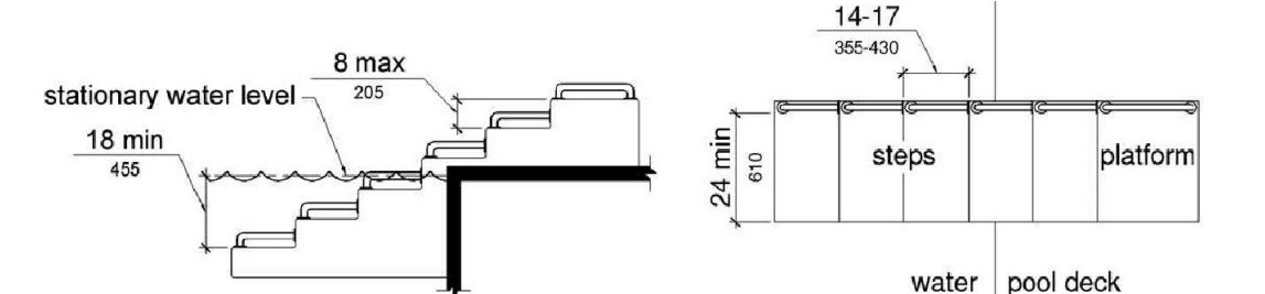
Figure 1009.5.4 Transfer Steps
