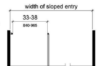
Figure 1009.3.3 Handrails for Sloped Entry
