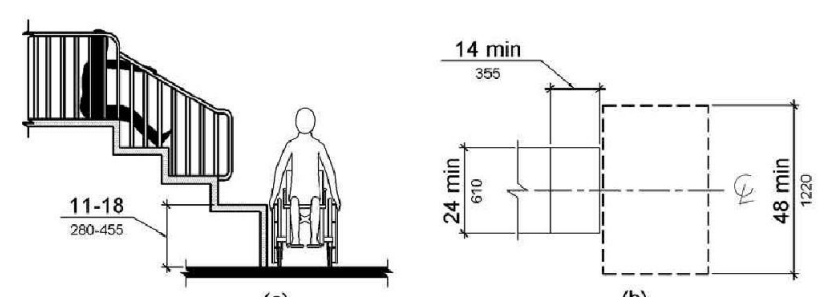
Figure 1008.3.1 Transfer Platforms
