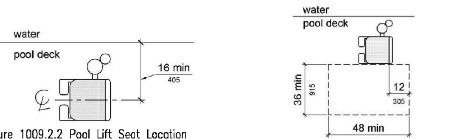
Figure 1009.2.3 Clear Deck Space at Pool Lifts
