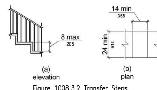
Figure 1008.3.2 Transfer Steps
