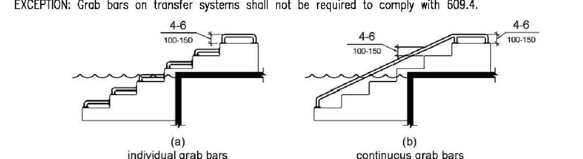
Figure 1009.5.7 Grab Bars
