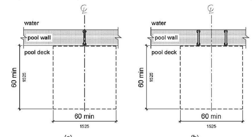
Figure 1009.4.1 Clear Deck Space at Transfer Walls
