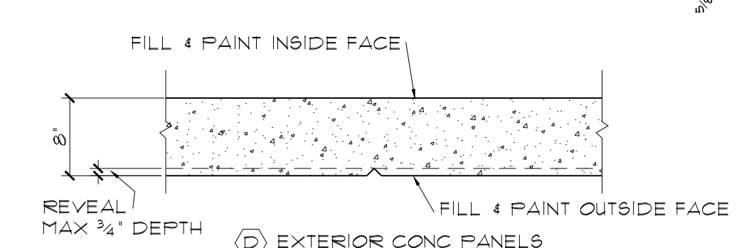
2 WALL TYPES SCALE: NTS
