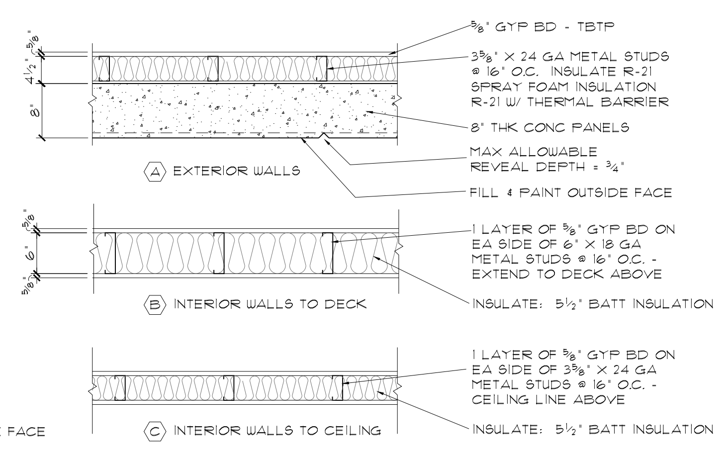
2 WALL TYPES SCALE: NTS
